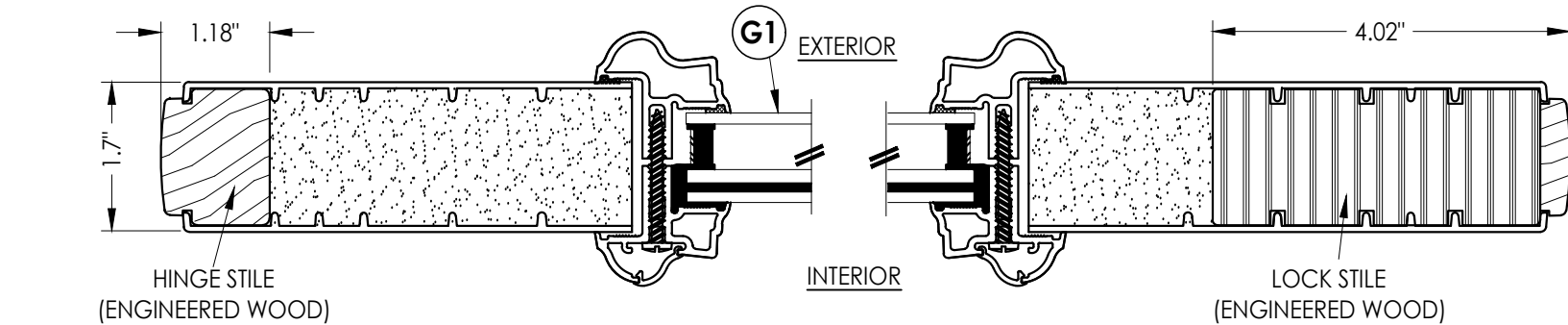
1 2 HORIZONTAL CROSS SECTION
